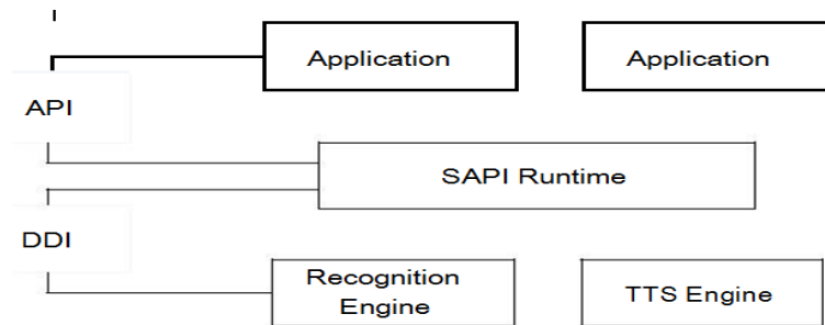
Figure 4. The structure of Speech SDK.
