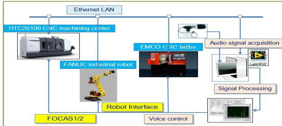
Figure 1. The hardware Structure of FMC.
