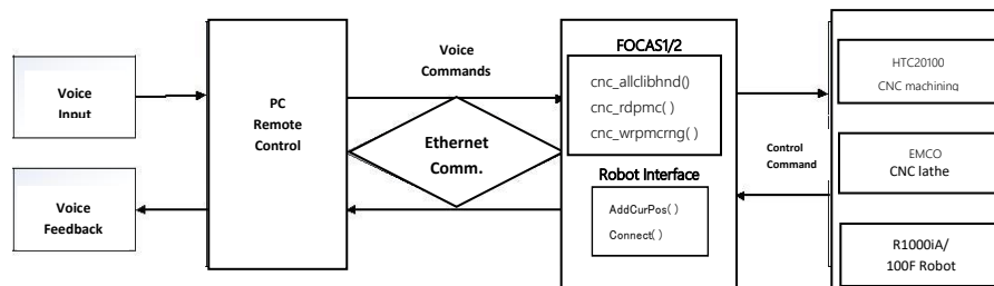
Figure 2. The system architecture of intelligent FMC based on voice control.
