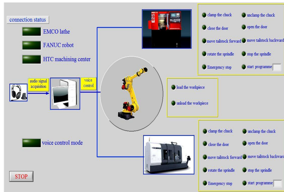
Figure 5. The voice control platform of intelligent FMC.
