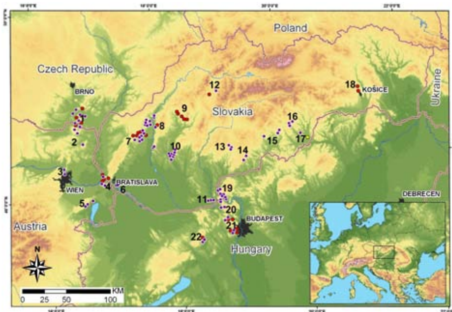
Fig. 1: Distribution of the analysed plots in the study area. Red circles indicate relevés of the Bromo-pannonici-Festucion pallentis , violet circles of the Festucion valesiaca , and the yellow circle the single relevé of the Cynosurion cristati . The numbers denote the geographic units in which the relevés were sampled. They are arranged in west-east and north-south directions. Czech Republic: Pavlovské vrchy Mts. (1); Austria: Weinviertel (2), Bisamberg (3), Hainburger Berge (4), Leitha-Gebirge (5); Slovakia: Podunajská rovina lowland (6), Malé Karpaty Mts. (7), Považský Inovec Mts. (8), Strážovské vrchy Mts. (9), Tríbeč Mts. – Zoborské vrchy Mts. (10), Hronská pahorkatina hills – Belianské kopce (11), Turčianska kotlina basin (12), Štiavnické vrchy Mts. (13), Krupinská planina hills (14), Lučenecká kotlina basin (15), Revúcka vrchovina hills – Drienčanský kras (16), Rimavská kotlina basin (17), Čierna hora Mts. (18); Hungary: Börzsöny Mts. (19), Visegrádi-hegység Mts and Pilis Mts. (20), Budai-hegysek Mts. (21), Vértes Mts. (22).
